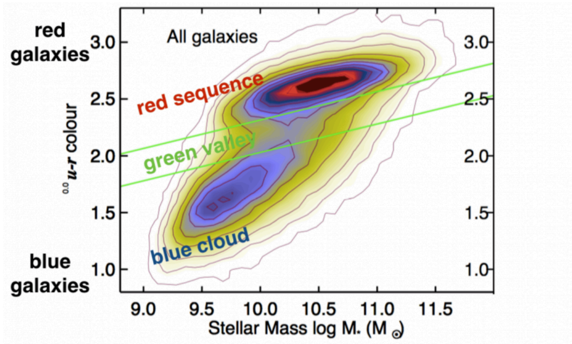
A plot of stellar mass and galaxy color. Our galaxy, the Milky Way Galaxy is currently in the “green valley”.
