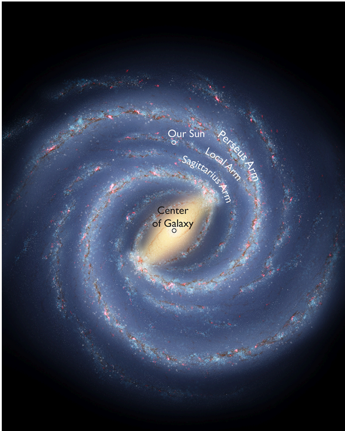
The closest spiral arms to our solar system within the Milky Way galaxy. The sun's location is provided for reference.
